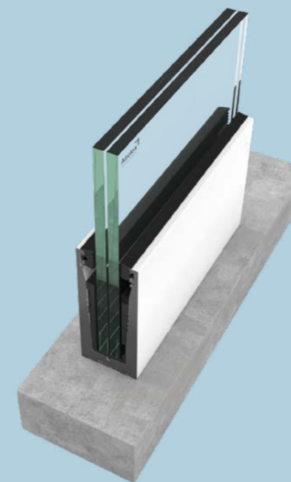
Glass railing
